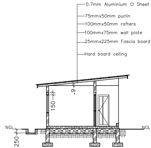
SECTIONAL ELEVATION (AO-AO) OF KITCHEN AND TOILET TYPE 2 QUARTER
