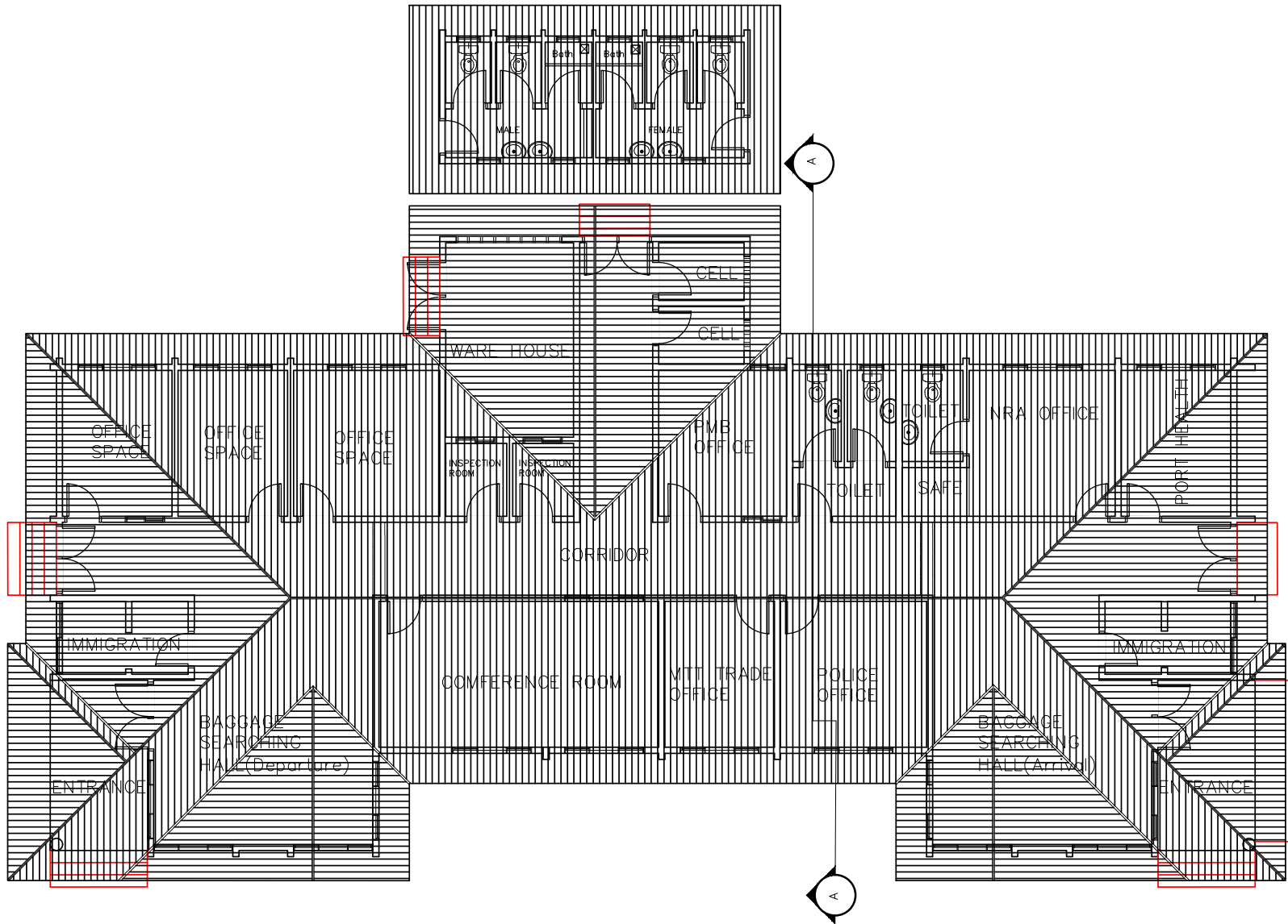
ROOF PLAN VIEW OF BEIDU CUSTOM BORDER OFFICE
