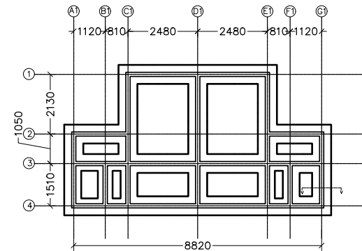
FOUNDATION LAYOUT PLAN OF TYPE 2 KITCHEN AND TOILET
