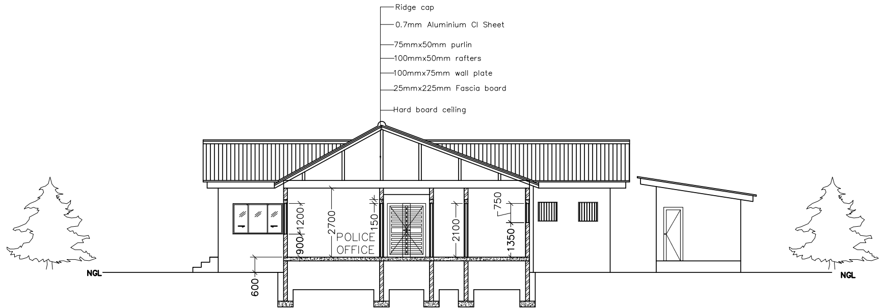
SECTION A-A ELEVATION VIEW OF BEIDU CUSTOM BORDER OFFICE
