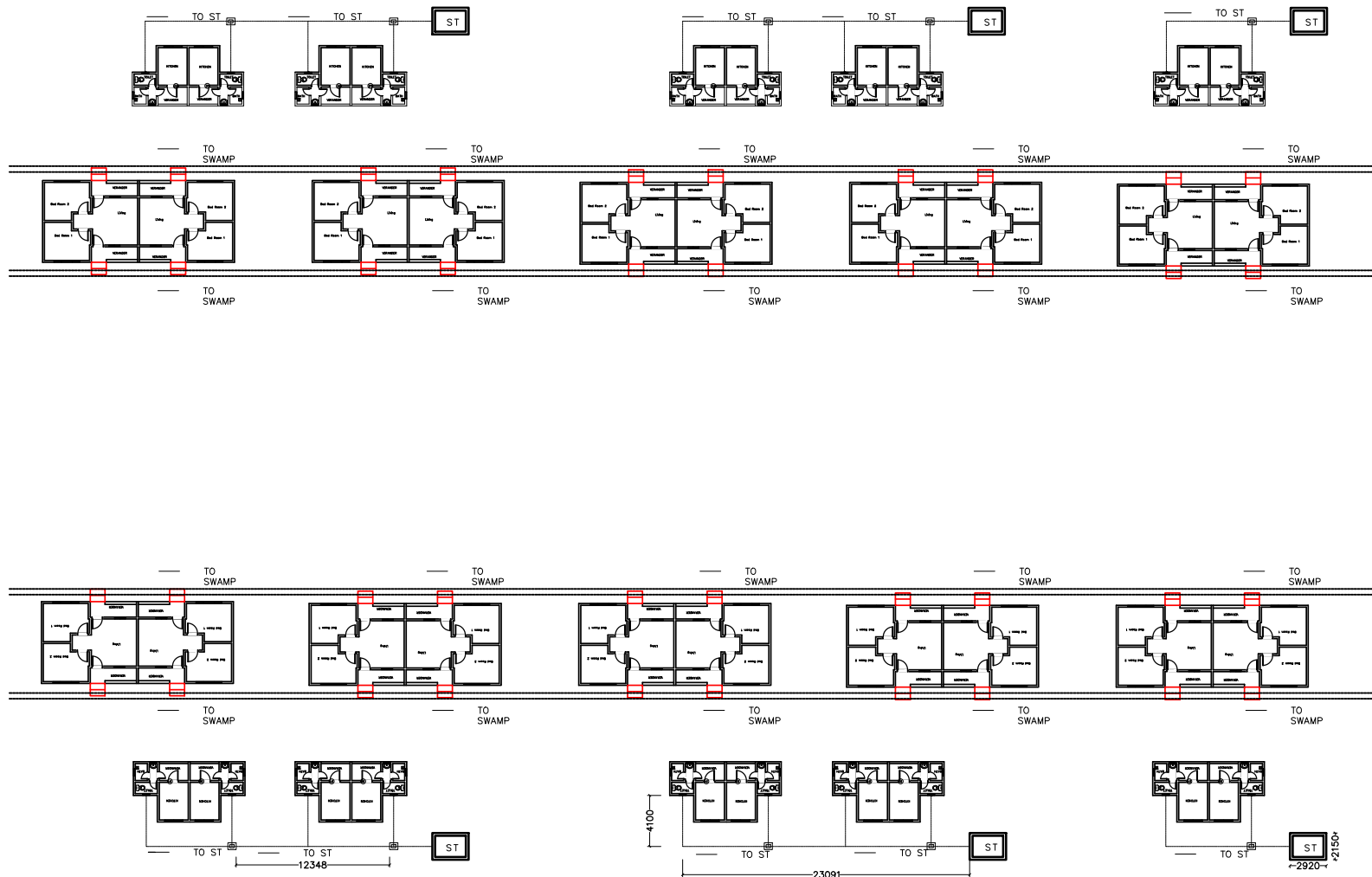
WASTE WATER AND SOIL LINE PIPE FOR TYPE 2 QUARTERS
