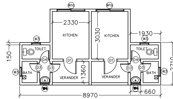
PLAN VIEW OF TYPE 2 KITCHEN AND TOILET
