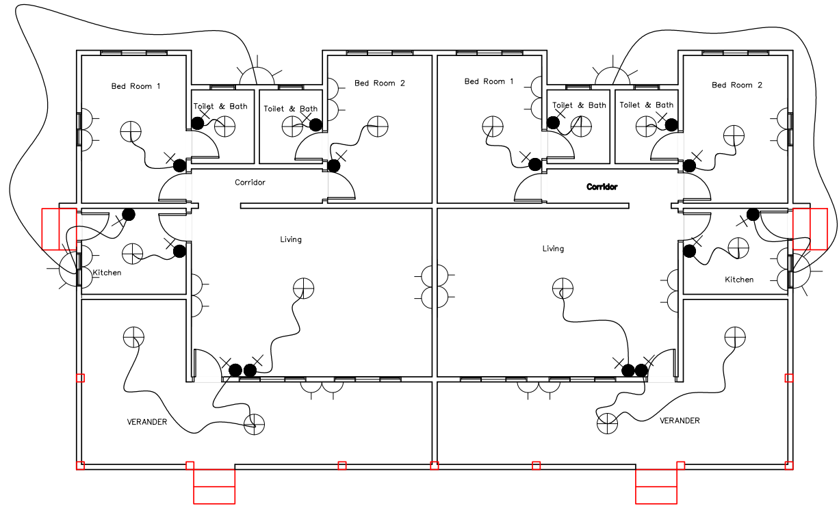
ELECTRICAL LAYOUT PLAN VIEW OF TYPE 1 QUARTER
