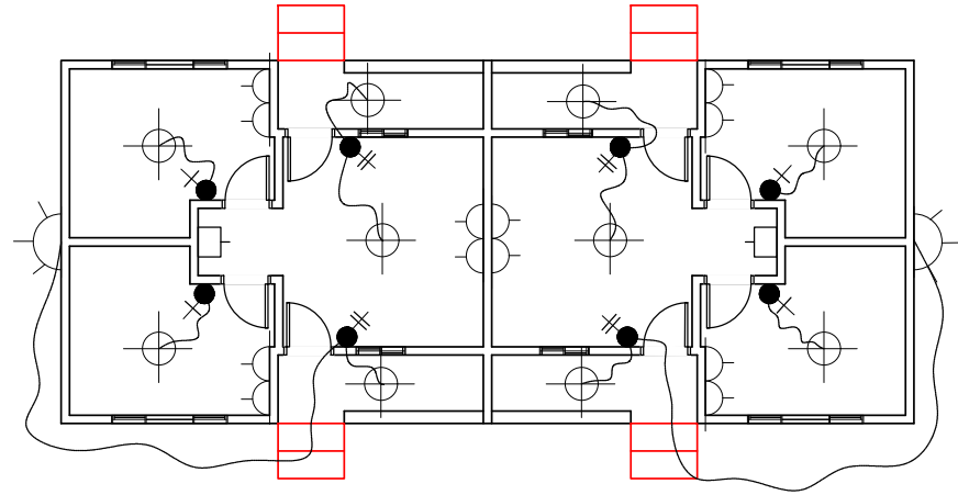
ELECTRICAL PLAN VIEW OF TYPE 2 QUARTER
