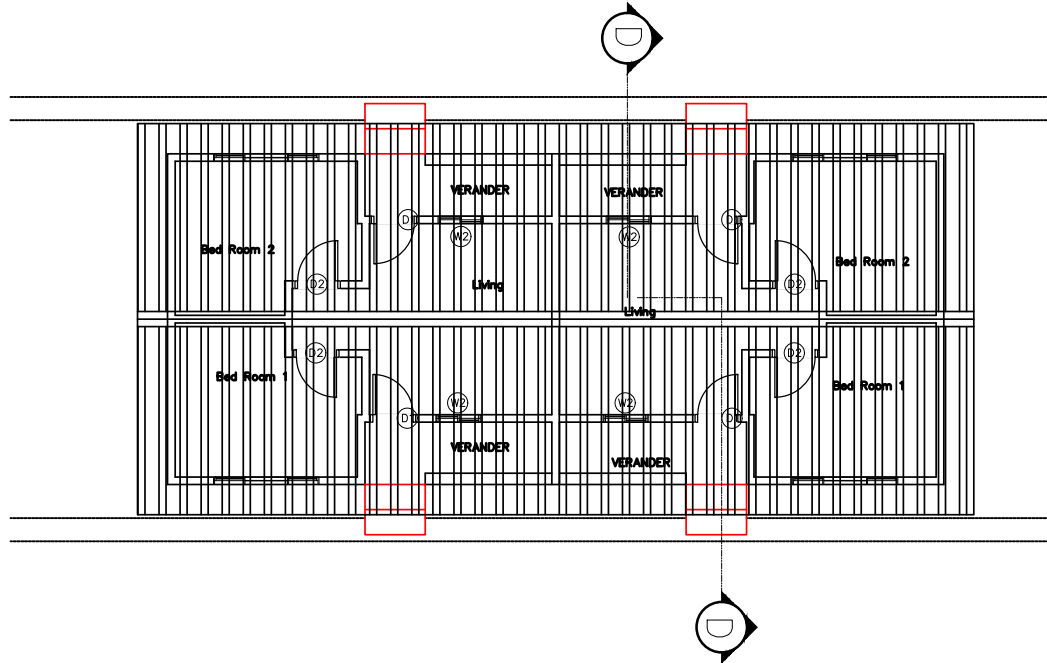
ROOF PLAN VIEW OF TYPE 2 QUARTER
