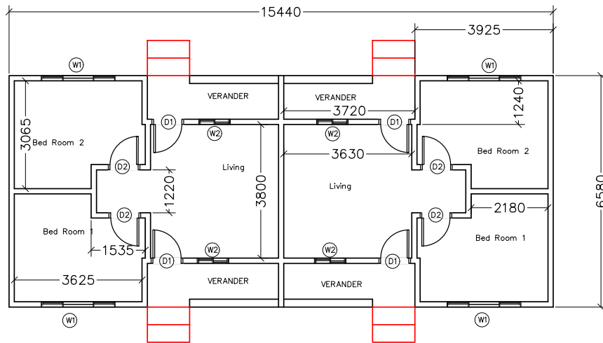
PLAN VIEW OF TYPE 2 QUARTER
