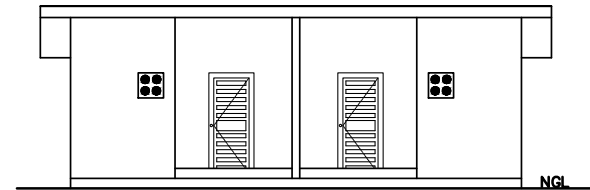
FRONT ELEVATION OF KITCHEN AND TOILET OF TYPE 2
