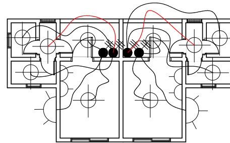
ELECTRICAL PLAN VIEW OF TYPE 2 QUARTER
