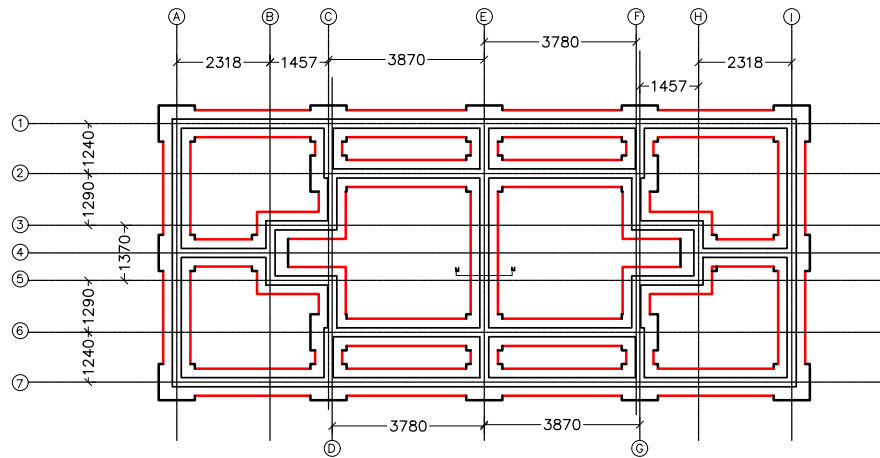
FOUNDATION LAYOUT PLAN OF TYPE 2 QUARTER
