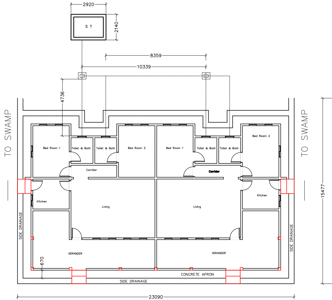
WASTE WATER AND SOIL LINE PIPE FOR TYPE 1 QUARTER
