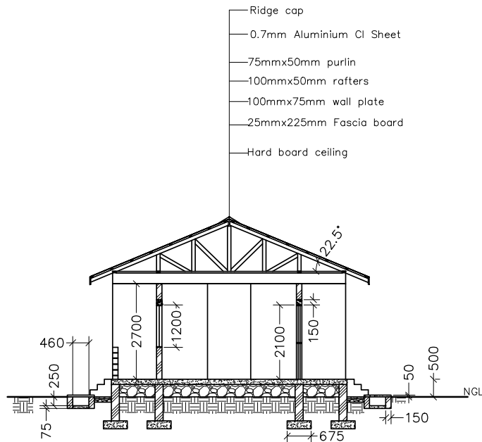
SECTIONAL ELEVATION D-D OF TYPE 2
