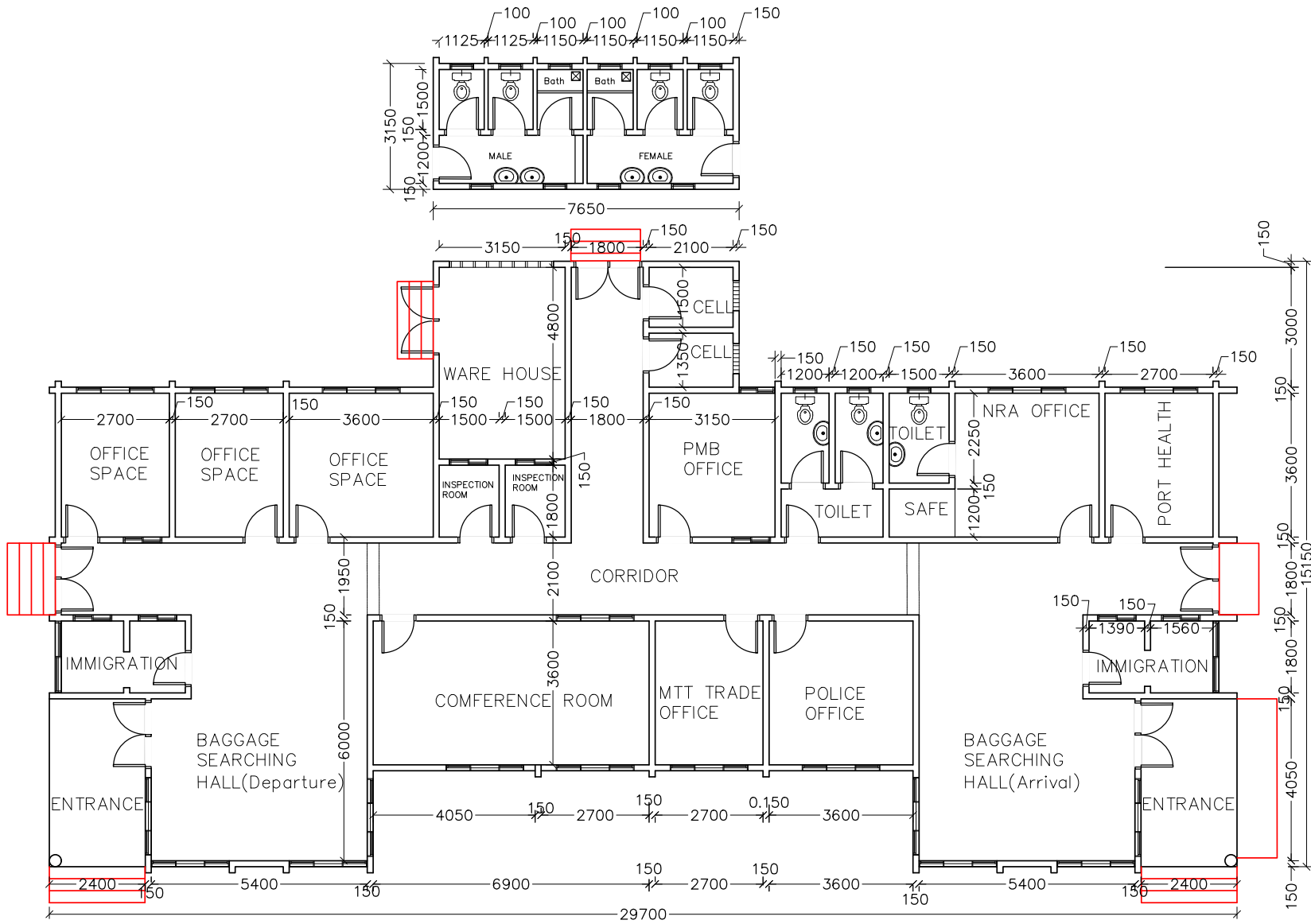
PLAN VIEW OF BEIDU CUSTOM BORDER OFFICE
