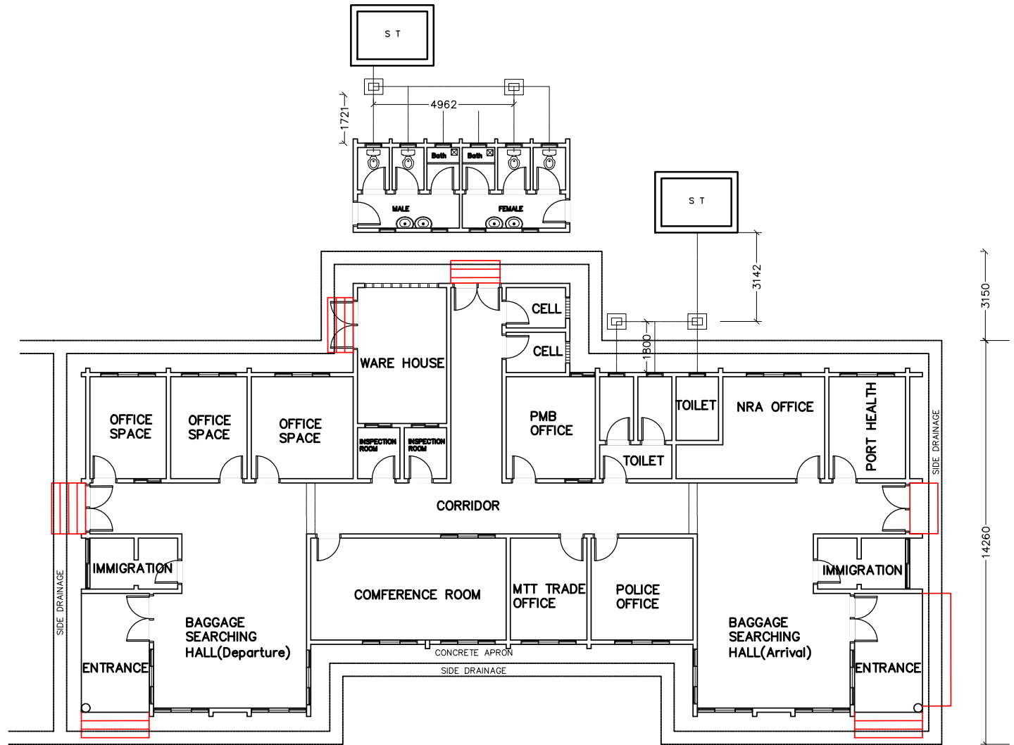
WASTE WATER AND SOIL LINE PIPE FOR OFFICE
