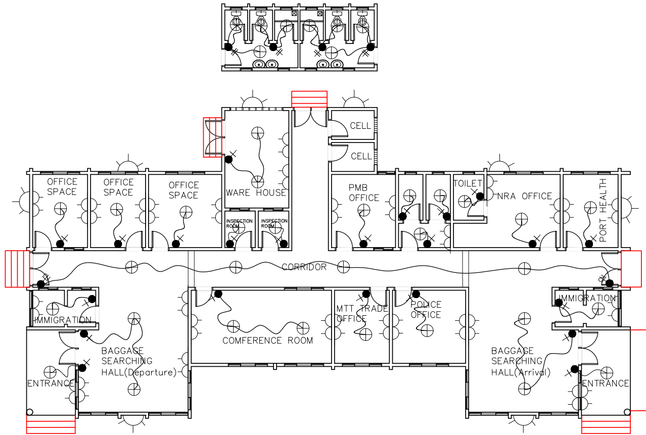
ELECTRICAL LAYOUT PLAN OF BEIDU CUSTOM BORDER OFFICE
