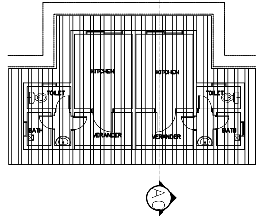
ROOF PLAN VIEW OF TYPE 2 KITCHEN AND TOILET
