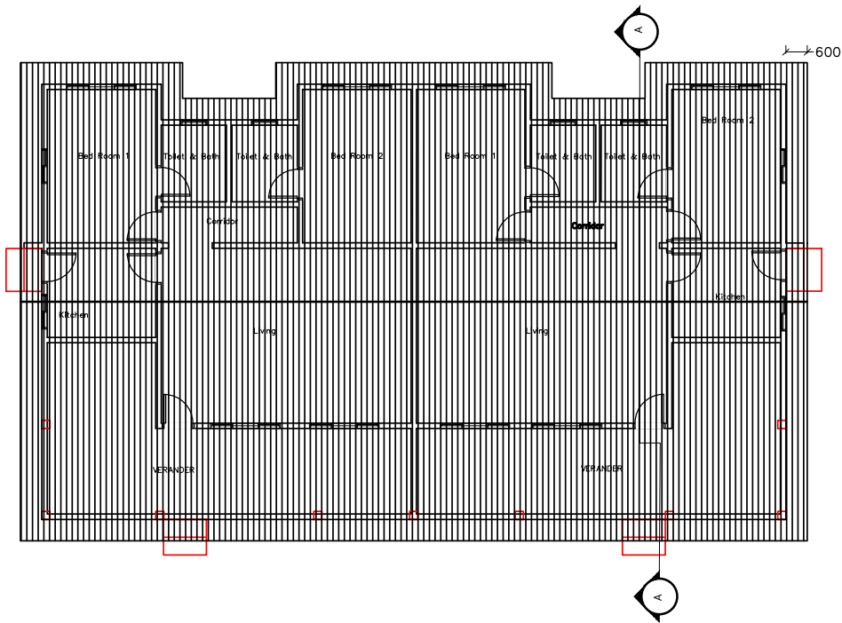
ROOF LAYOUT PLAN OF TYPE 1 QUARTER
